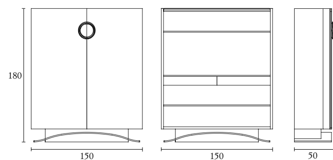
Cod. HAUSSBAR cm 150 x 50 x 180 - inch 59 x 19.6 x 70.8
