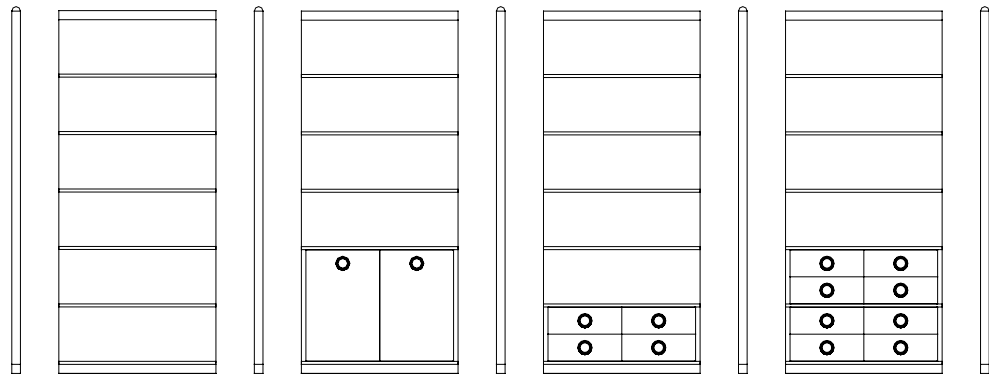
Cod. HMATBI55CV / HMATBI55CL / HMATBI55C cm 55 x 46 x h 240 - inch 21.6 x 18.1 x 94.4
