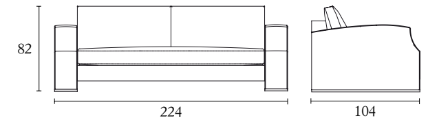
Cod. ANTOI280SM cm 284 x 104 x h 82 - inch 110 x 40.9 x 32.2
