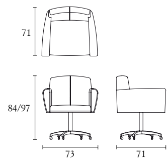
Cod. HAFAUBURP cm 73 x 71 x h 84/97 - inch 28.7 x 27.9 x 33/38.2
