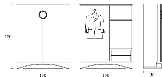
Cod. HAUSSVIT cm 150 x 50 x 180 - inch 59 x 19.6 x 70.8
